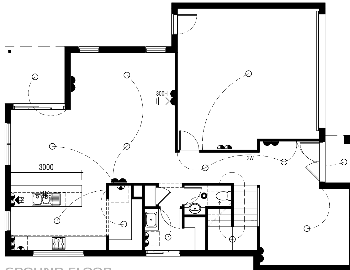
GROUND FLOOR
