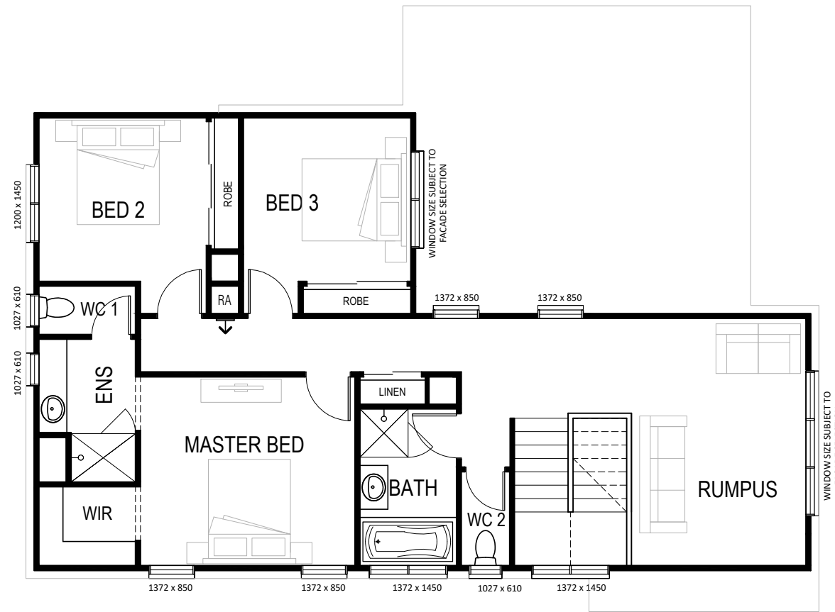
FIRST FLOOR
